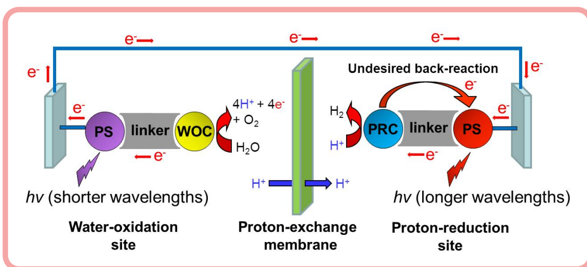
Figure 3 Schematic representation of a tandem photoelectrochemical cell (PEC) for water splitting (see text for explanation). (WOC = water oxidation catalyst; PRC = proton ( H^+ ) reduction catalyst, h\nu = solar radiation). 4
